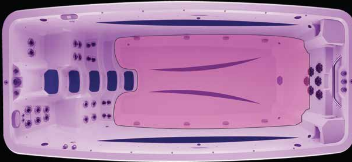
Marquis Swim Spa ATV-17 SPORT Shell Dimensions: 204" L x 61" H x 89.5" W
